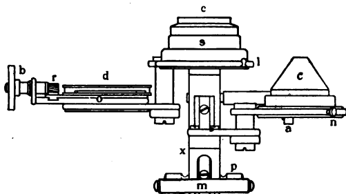
Fig. 51b. Complete Substage. Front view, with condenser and lower iris diaphragm swung out of optical axis.
